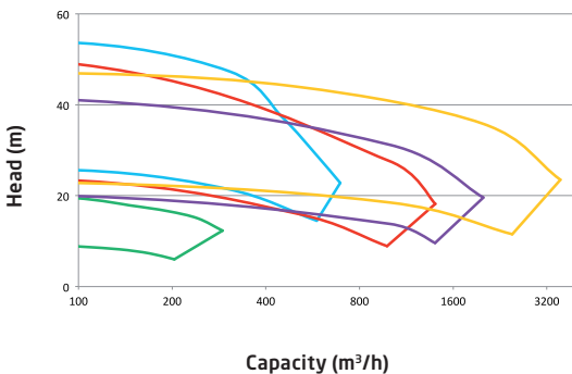
Pump Performance Curve
